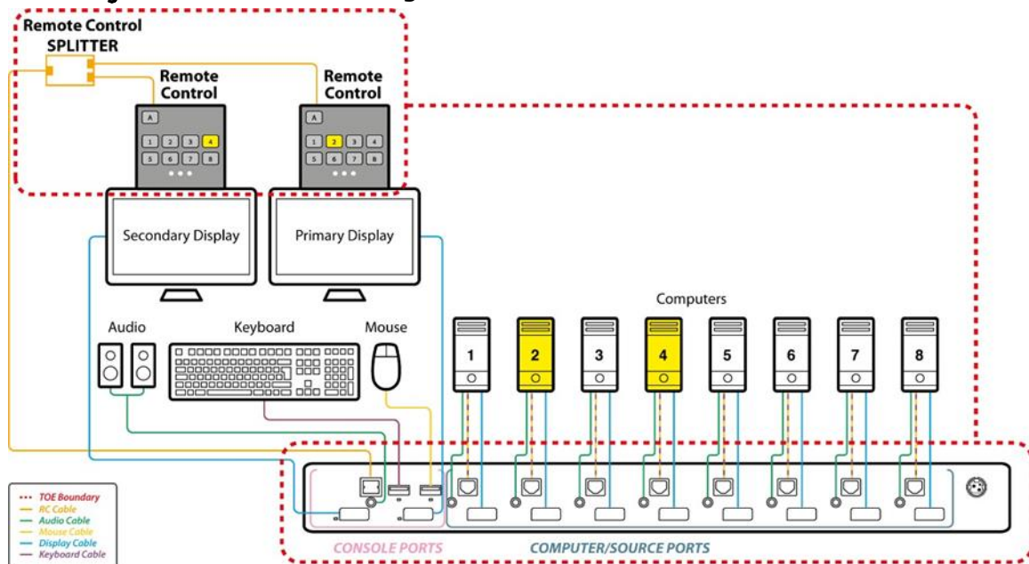
Figure 1: – Evaluated Configuration for KVM and Matrix Switches.
