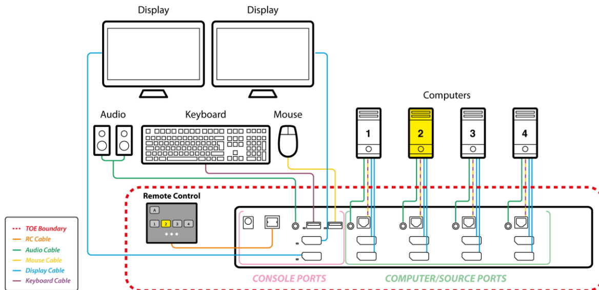
Figure 1: – Evaluated Configuration for KVM and Matrix Switches.
